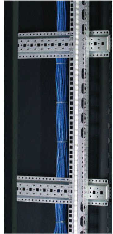
Zinc mounting angle available for binding wires
